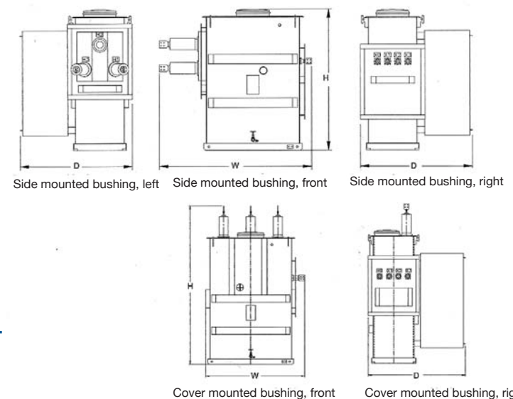
35 kV Class
